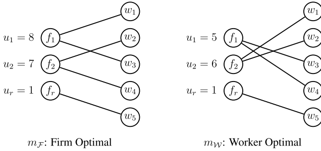
FIGURE 1. Stable matchings.
