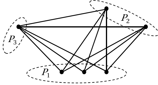
Figure 1: A complete three-partite graph
