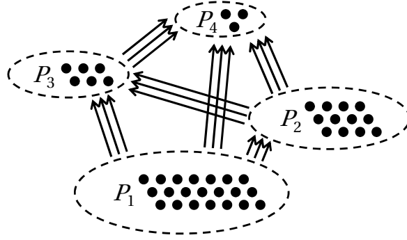
Figure 2: Schematic illustration of a directed complete four-partite graph with different-sized partite sets and upward linking
