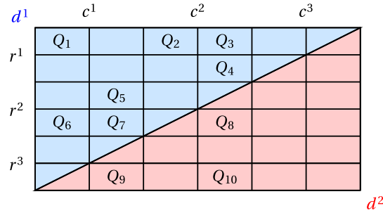
FIGURE 3. The state space \Omega and information partitions.
